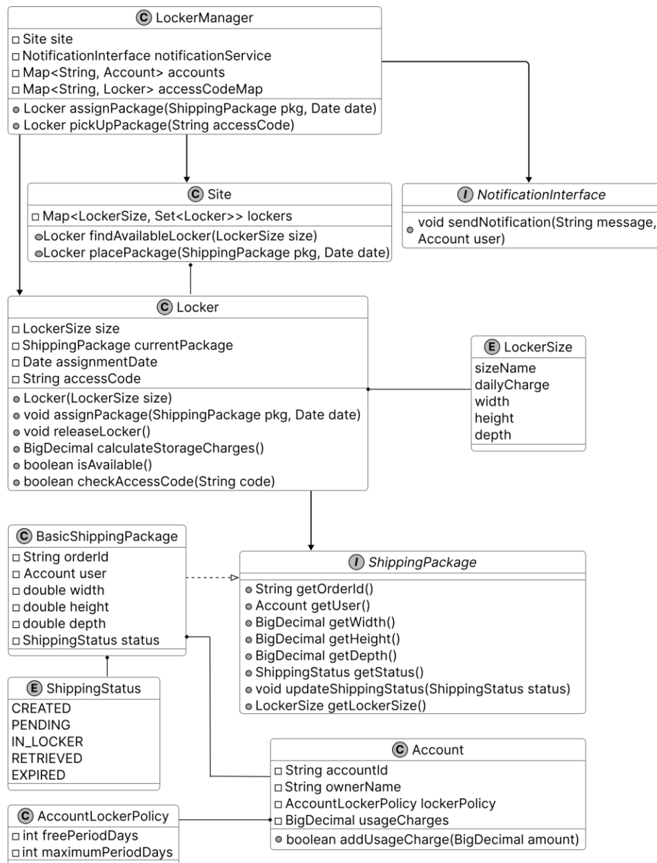
Class Diagram of Locker Service
